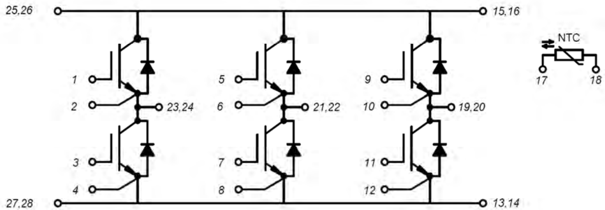
Figure 14. Circuit Diagram
