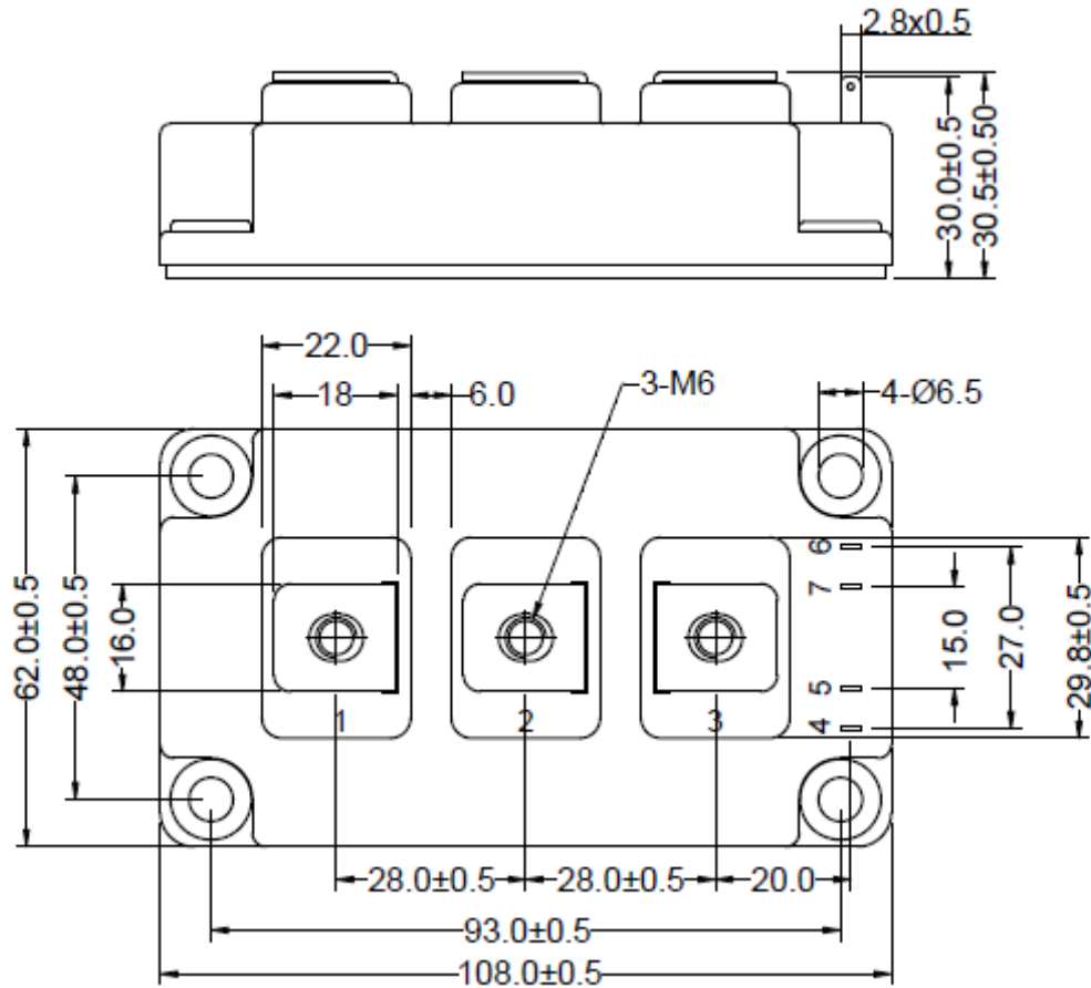
Dimensions (mm) Figure12. Package Outline
