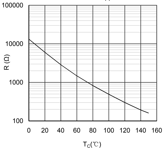
Figure 14. NTC Characteristics
