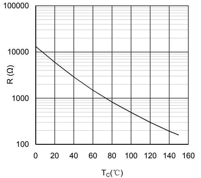
Figure 12. NTC Characteristics
