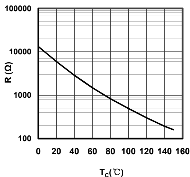
Figure 14. NTC Characteristics
