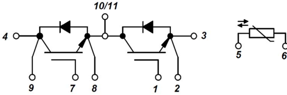
Figure 14. Circuit Diagram
