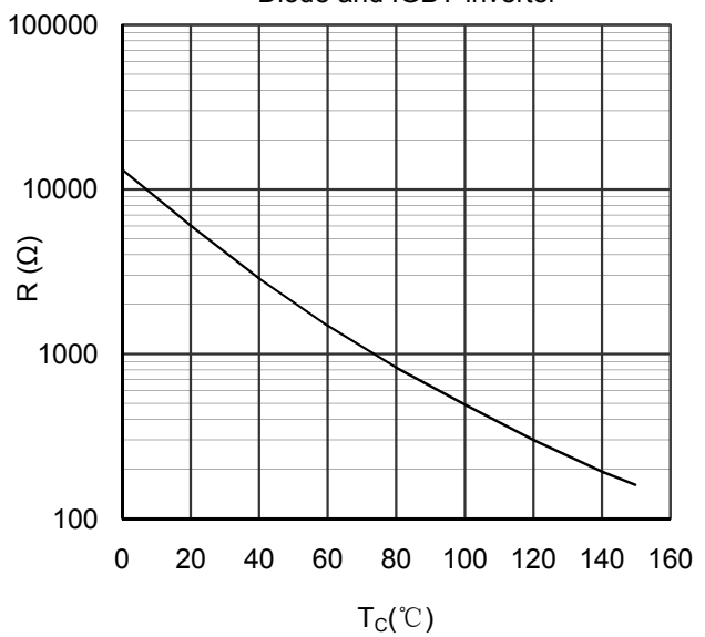
Figure 13. NTC Characteristics
