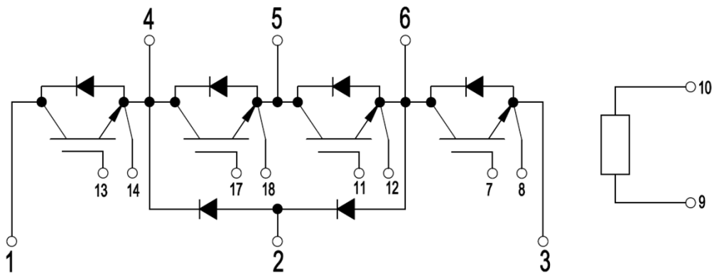
Figure 13. Circuit Diagram
