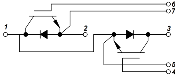
Figure 13. Circuit Diagram
