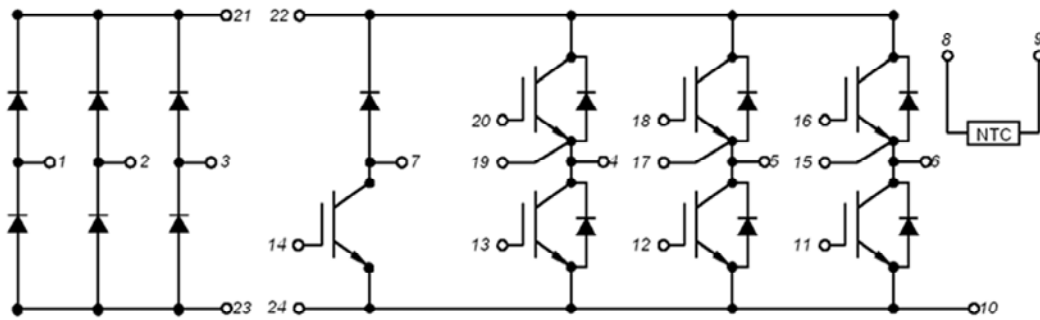
Figure 17. Circuit Diagram
