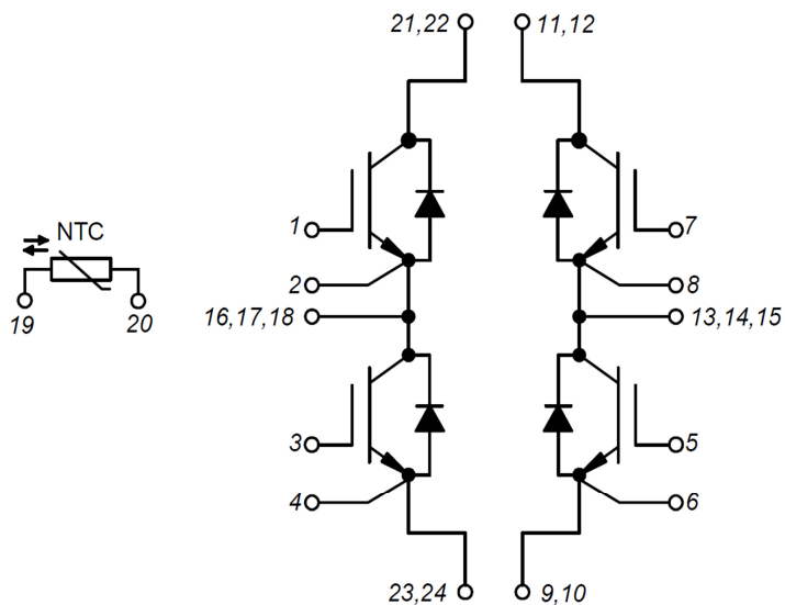
Figure 14. Circuit Diagram
